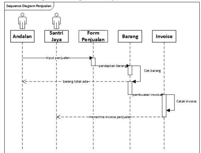
Gambar 4.1 Sequence Diagram Penjualan
