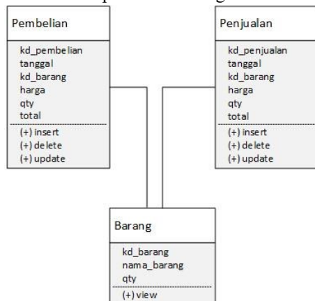
Gambar 4.3 Class Diagram Andalan Poultry Shop dan Santri Jaya Farm
