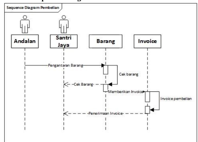
Gambar 4.2 Sequence Diagram Pembelian
