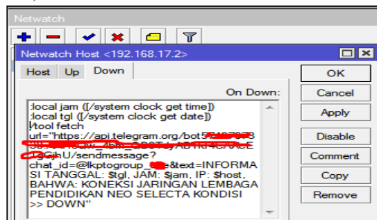
Gambar 23. Script Down Netwatch
